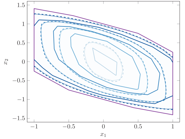
Fig. 4. (— 0.1, — 0.5, — 1, and — 2)–Contours of M (continuous lines), M' (dotted lines), and M^* (dashed lines).
