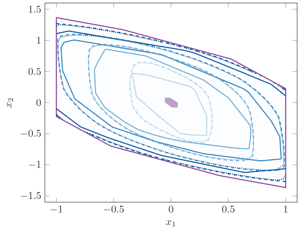
Fig. 7. (■ 0.1, ■ 0.5, ■ 1, and ■ 2)-Contours of M (continuous lines), M' (dotted lines), and M^* (dashed lines). The 0-sublevel set (■) corresponds, for all functions, to X_s .
